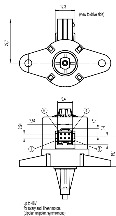
Connector D for Molex C-Grid III 90142-0006
