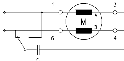
Series circuit 110 V (only for connector N)
