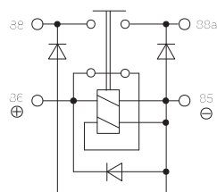
Suppression diode Polarity protection
