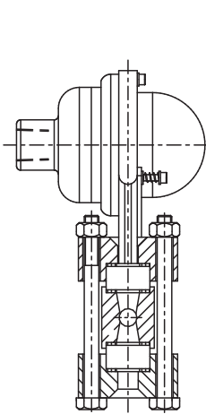
Sectional view of illuminator
